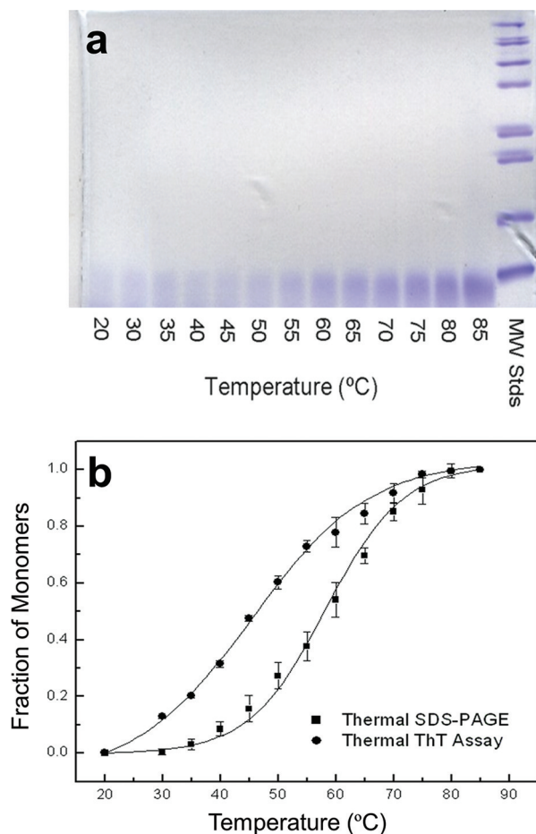
Figure 4. Thermal stability of SAA2.2 fibrils monitored by GCL/SDS-PAGE and ThT fluorescence. (a) Representative gel showing the extent of monomer populated after cross-linking at various temperatures. (b) The gel data were analyzed by quantifying the bands and then plotting the relative fraction of SAA2.2 monomer versus temperature (■). The thermal denaturation of SAA2.2 fibrils was also monitored by the disappearance of the ThT fluorescence (●). The estimated transition midpoints for the gel and ThT data were ~58 and ~48 °C, respectively. Error bars are based on triplicate experiments.
