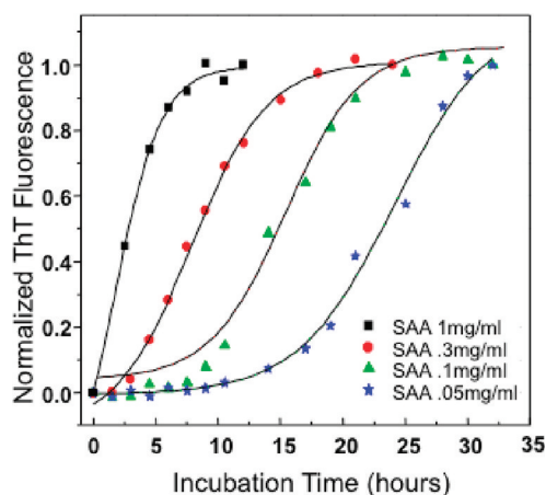
Figure 2. Formation of SAA2.2 amyloid fibrils monitored by thioflavin T fluorescence. The curves represent the changes in ThT fluorescence as a function of time upon binding to SAA2.2 fibrils formed at different protein concentrations (20 mM Tris-HCl, pH 7.4) and 37 °C. The presence of a variable lag phase is consistent with a nucleation/seedling mechanism.
