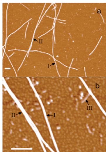
Figure 1. AFM images of mature SAA2.2 fibrils formed after incubation of SAA2.2 (20 mM Tris-HCl, pH 7.4) at 37 °C for 2–3 weeks. Several types of structures are evident, including (I) fibrils with 1–2 nm in height and of variable length; (II) several type I fibrils joined together to form higher-ordered fibrils; and (III) short protofibrils formed by interaction of spherical oligomers. Scale bars in (a) and (b) represent 500 and 200 nm, respectively.
