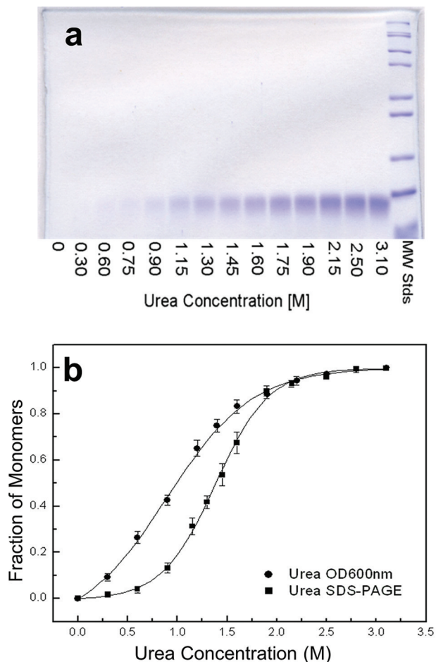
Figure 5. Urea-induced denaturation of SAA2.2 fibrils monitored by GCL/SDS-PAGE and light scattering. (a) Representative gel data showing the extent of monomer populated after cross-linking at various concentrations of urea. (b) Gel data analyzed by plotting the density of monomer bands against urea concentrations (■). The urea-induced denaturation of SAA2.2 fibrils was also monitored by light scattering at 600 nm (●). The estimated transition midpoints for the gel and OD_{600} data were ~1.4 and ~1.0 M, respectively. Error bars are based on triplicate experiments.
