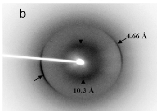
Figure 3. (a) Far-UV CD spectrum and (b) X-ray diffraction of SAA2.2 amyloid fibrils. The CD spectrum of SAA2.2 fibrils contains a minimum at 218 nm and maximum at 195 nm, consistent with the significant presence of \beta -sheet structure. Both the fibril solution and hexameric SAA2.2 were diluted to a final concentration of 0.1 mg/mL in PB buffer (pH 7.4). X-ray fibril diffraction pattern from SAA2.2 shows a classic amyloid-like cross-beta pattern with diffraction signals at 4.66 Å (arrows) and 10.3 Å (arrow heads).
