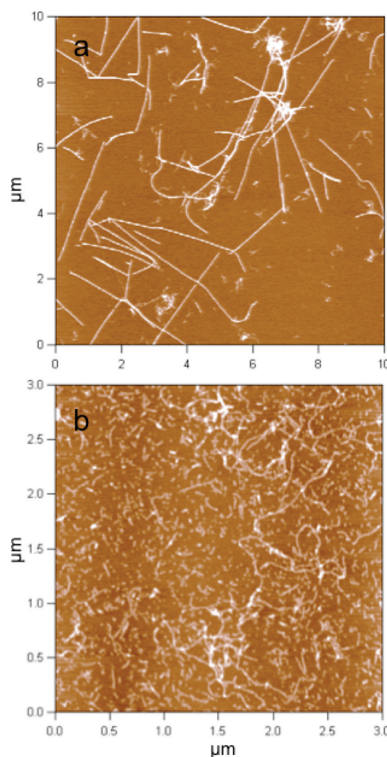
Figure 6. Thermal denaturation of SAA2.2 amyloid fibrils examined by AFM. (a) Mature fibrils of SAA2.2 formed by incubating an SAA2.2 sample ( \sim 2.5 mg/mL in 20 mM Tris buffer, pH 7.4) at 37 °C for 2 weeks. Long fibrils interacting with each other are clearly seen before thermal denaturation. (b) Mature SAA2.2 fibrils were incubated at 40, 45, and 50 °C for 0.5 h at each temperature in sequential order. The thermally denatured fibrils were then diluted 20 times and prepared on mica for AFM imaging in air as described in the Experimental Procedures section. AFM image shows the dissociation of mature fibrils into short fibrils and protofibrils.
